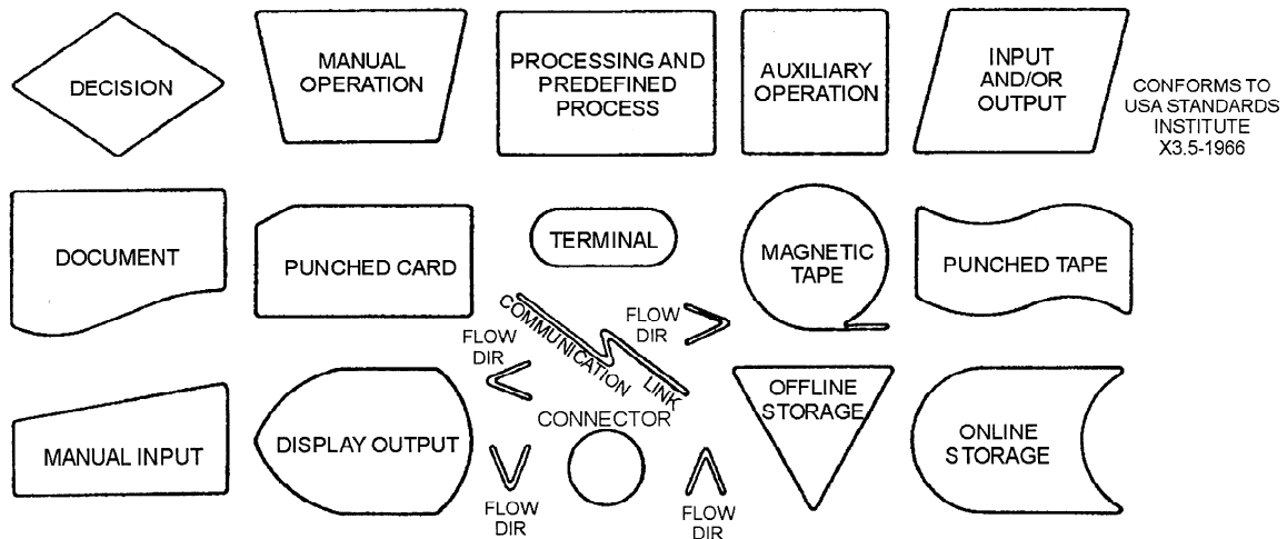
Figure 3-4.—Flowchart template.
