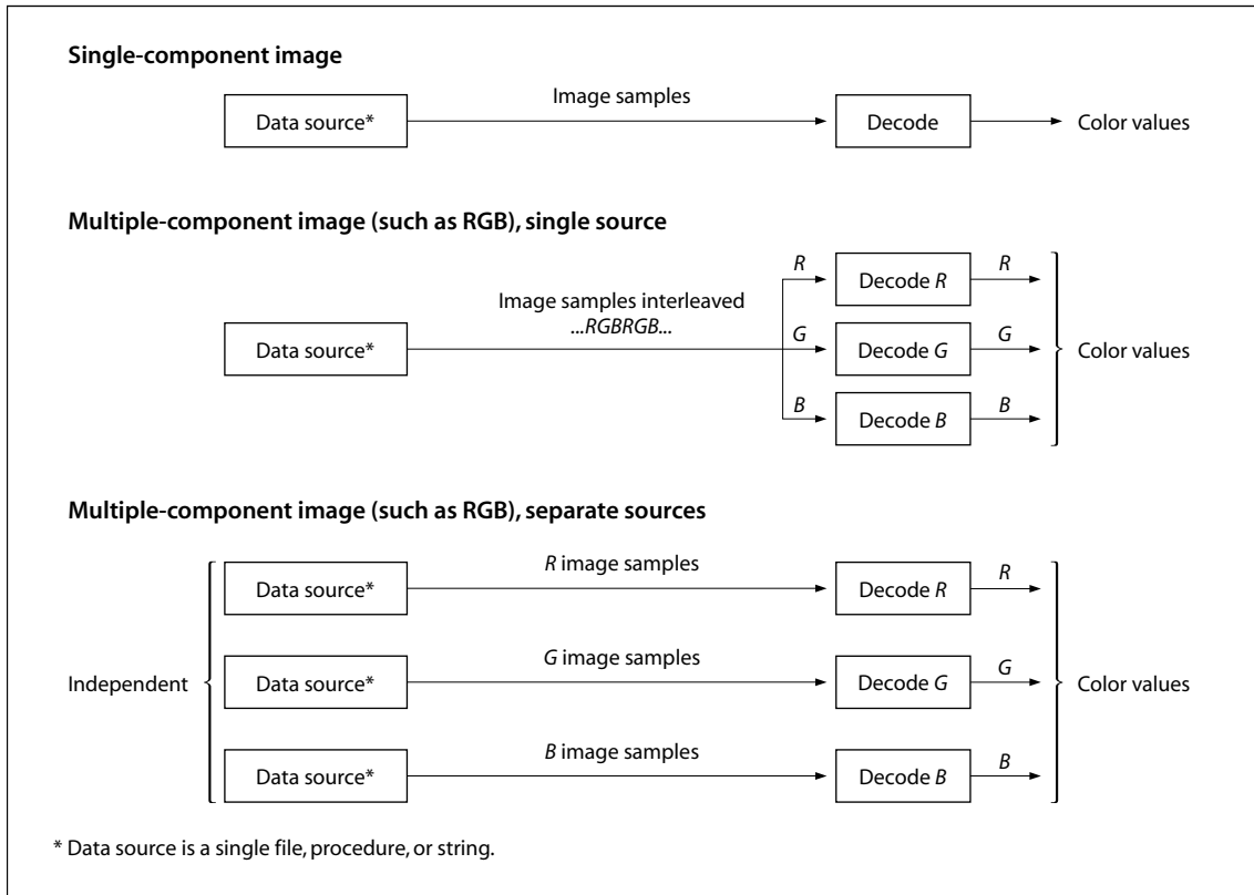
FIGURE 4.22 Image data organization and processing
