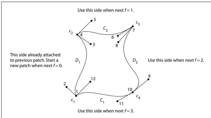
FIGURE 4.18 Color values and edge flags in Coons patch meshes
