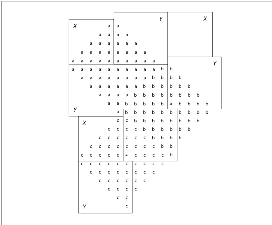
FIGURE 7.4 Halftone cell and two squares tiled across device space
