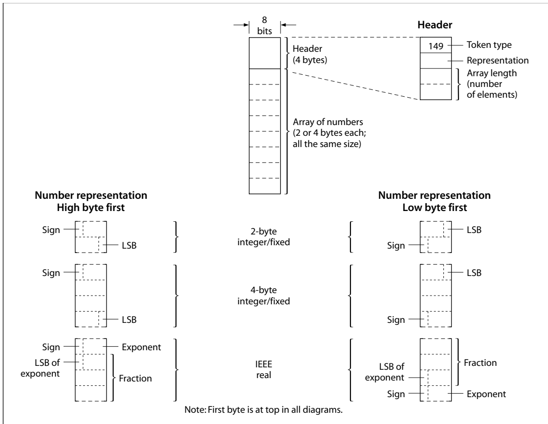
FIGURE 3.2 Homogeneous number array
