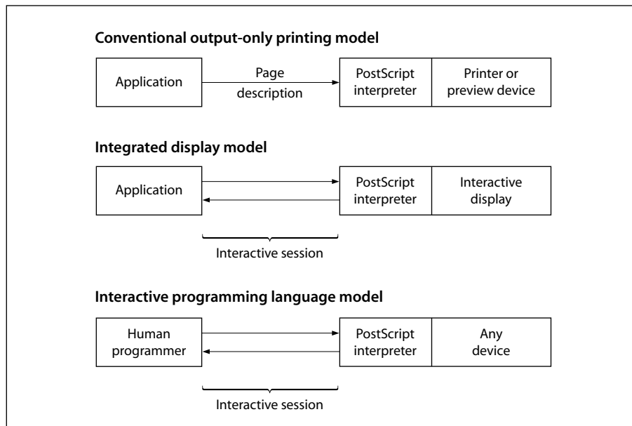
FIGURE 2.1 How the PostScript interpreter and an application interact
