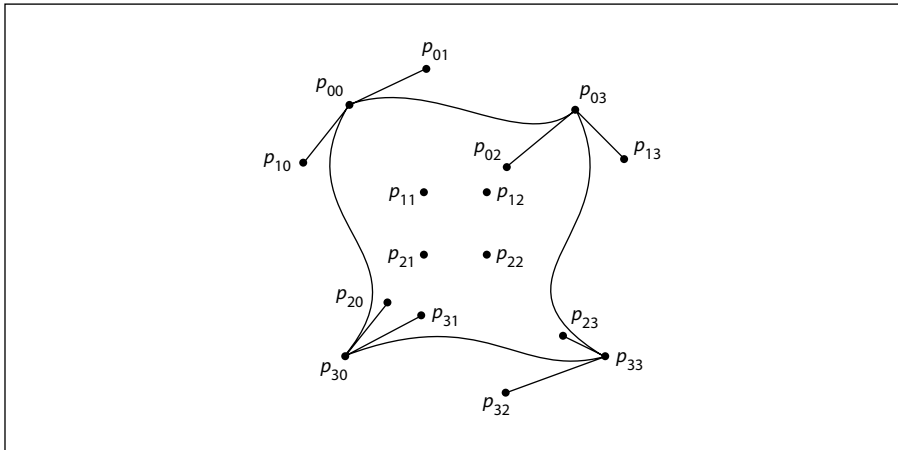
FIGURE 4.20 Control points in a tensor-product mesh
