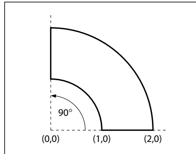
FIGURE 8.3 arcn operator example
