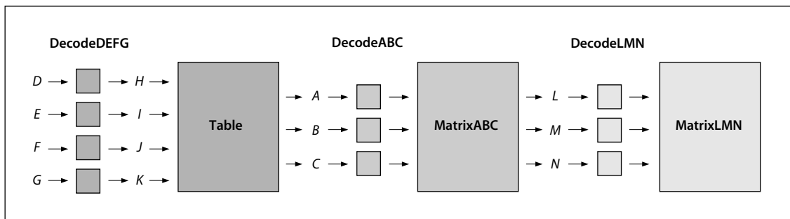
FIGURE 4.9 CIEBasedDEFG pre-extension to the CIEBasedABC color space
