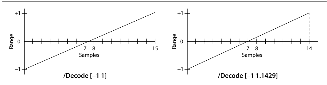
FIGURE 3.1 Mapping with the Decode array
