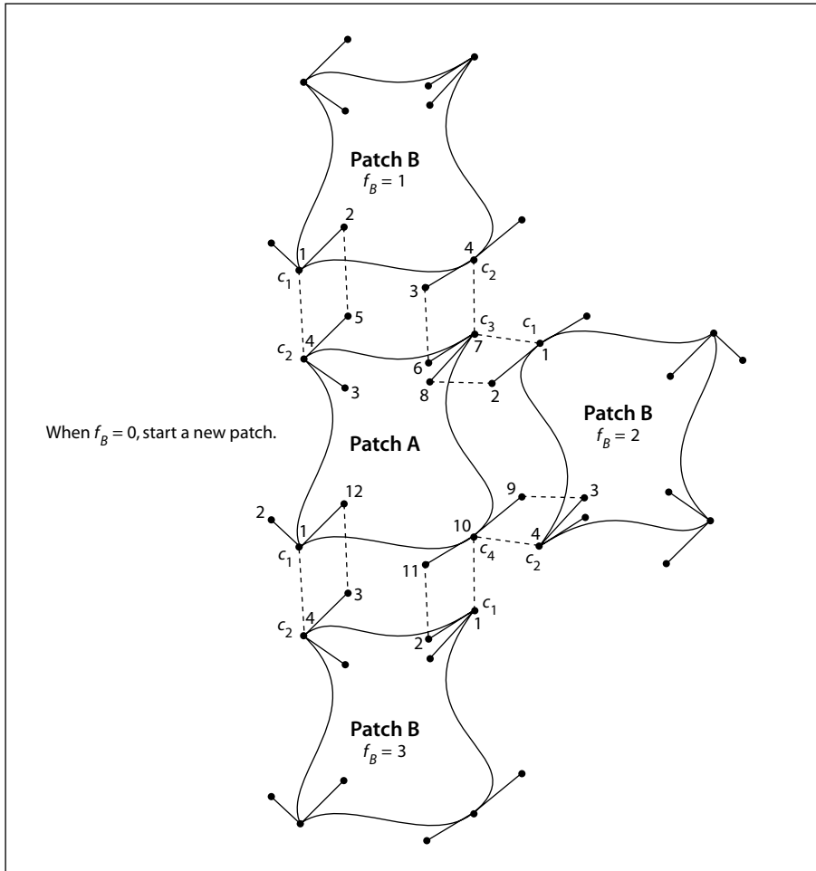
FIGURE 4.19 Edge connections in a Coons patch mesh
