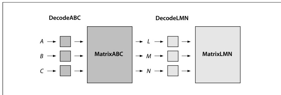
FIGURE 4.7 Component transformations in the CIEBasedABC color space
