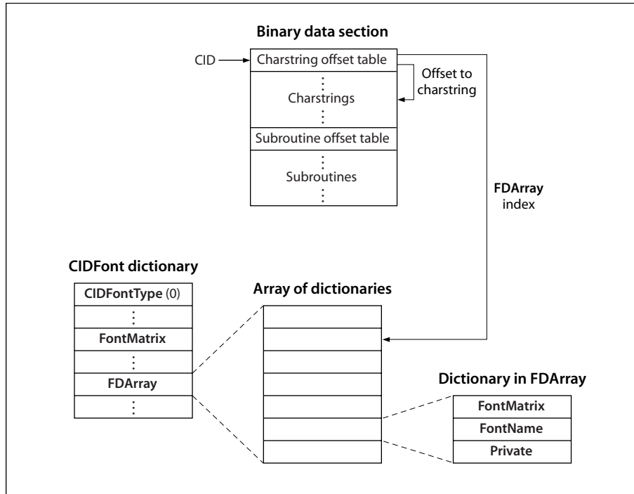
FIGURE 5.11 Type 0 CIDFont character processing
