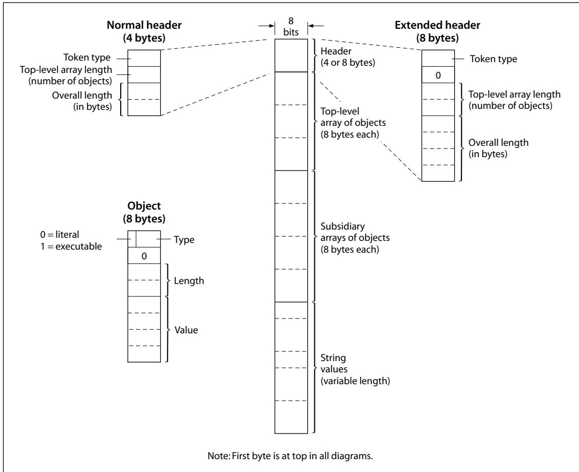
FIGURE 3.3 Binary object sequence
