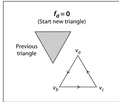
FIGURE 4.12 Starting a new triangle in a free-form Gouraud-shaded triangle mesh
