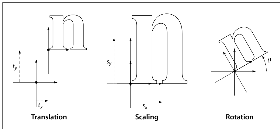
FIGURE 4.2 Effects of coordinate transformations
