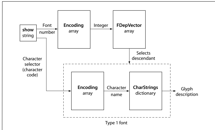
FIGURE 5.9 Composite font mapping example
