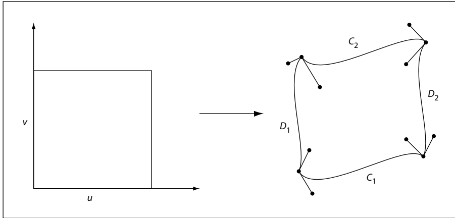
FIGURE 4.16 Coordinate mapping from a unit square to a four-sided Coons patch
