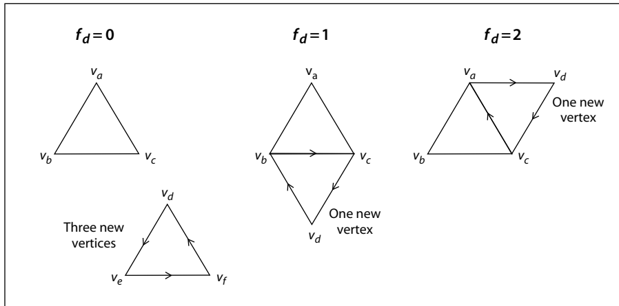
FIGURE 4.13 Connecting triangles in a free-form Gouraud-shaded triangle mesh
