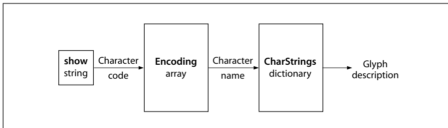
FIGURE 5.5 Encoding scheme for Type 1 fonts
