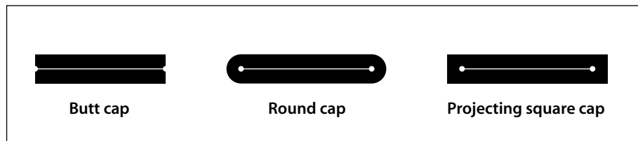
FIGURE 8.9 Line cap parameter shapes
