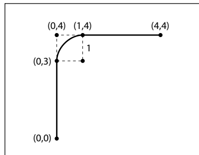
FIGURE 8.5 arct operator example
