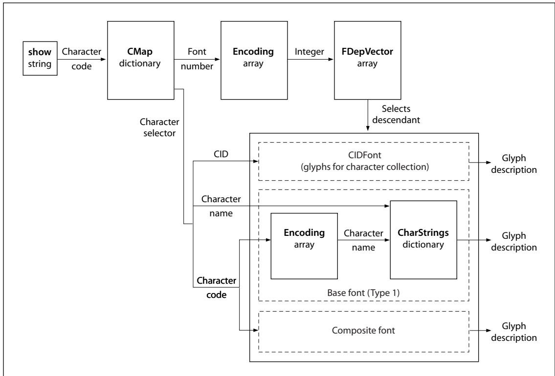
FIGURE 5.10 CID-keyed font basics
