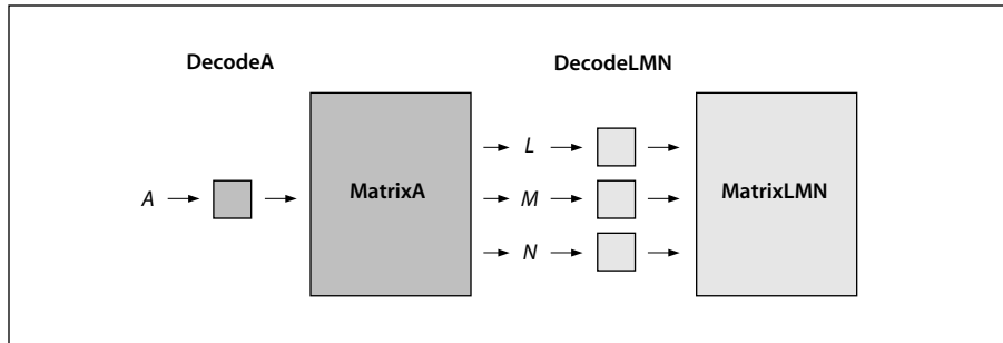
FIGURE 4.8 Component transformations in the CIEBasedA color space
