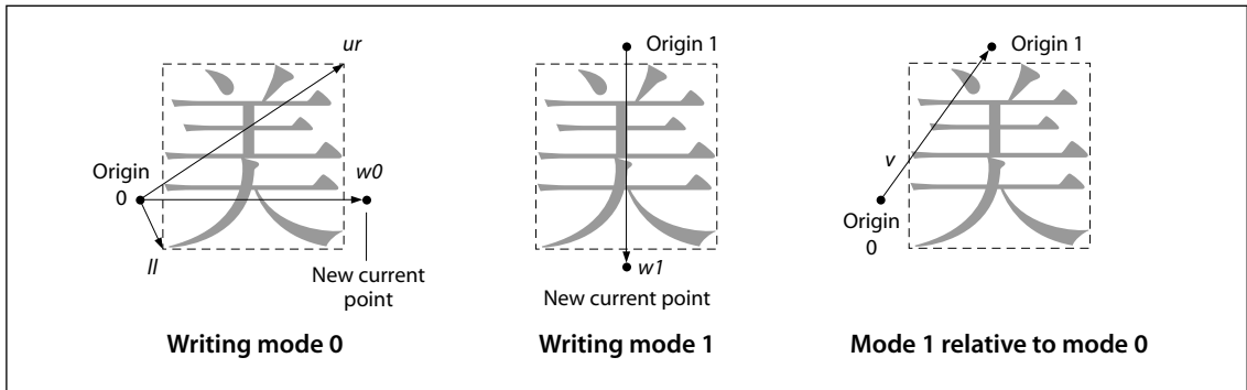
FIGURE 5.7 Relationship between two sets of metrics
