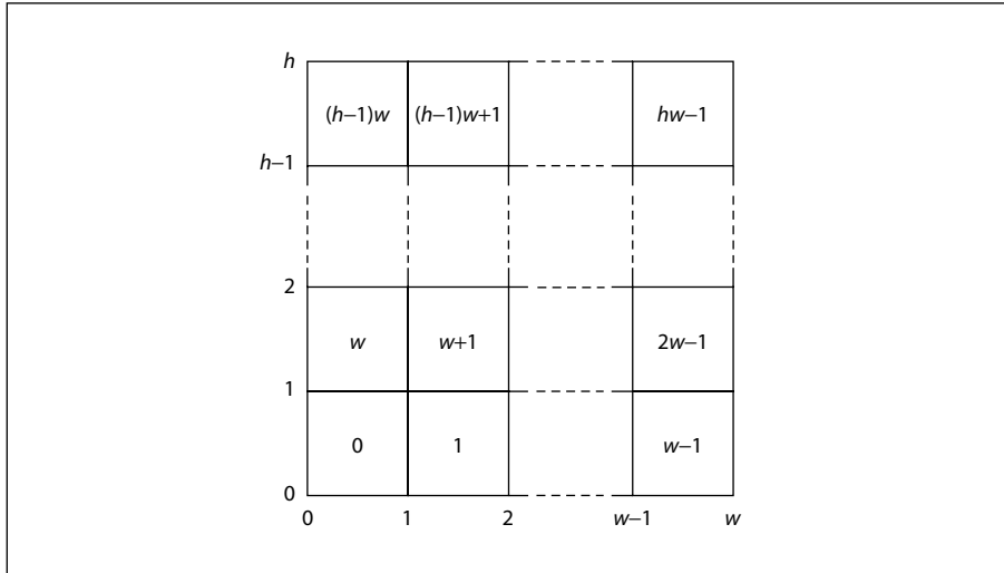
FIGURE 4.23 Source image coordinate system
